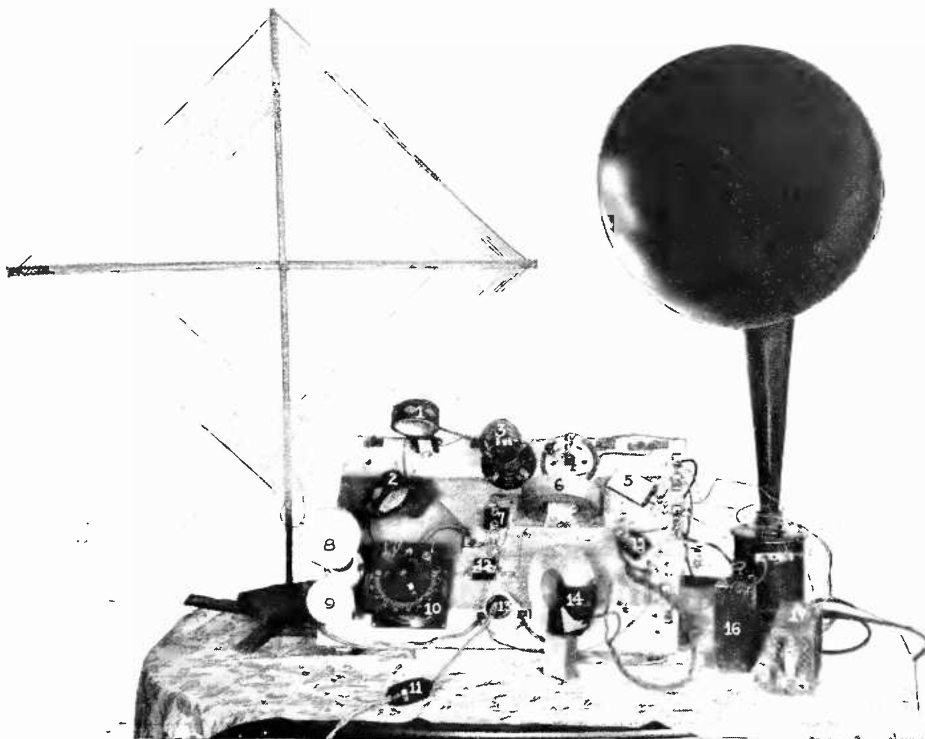
MR. ROBERTS' BATTERYLESS LOOP SET
